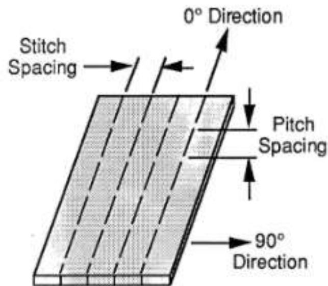
Figure 3. Depiction of Boeing's Stitched Uniweave.
