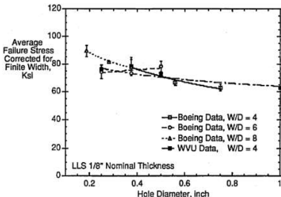
Figure 12. Effect of Hole Diameter on Open Hole Tension Strength. LLS 2-D Braid at 1/8" Nominal Thickness.
