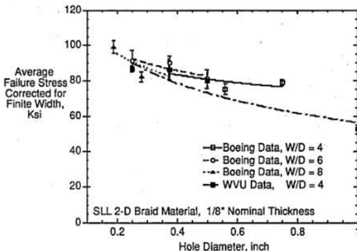
Figure 10. Effect of Hole Diameter on Open Hole Tension Strength. SLL 2-D Braid at 1/8" Nominal Thickness.
