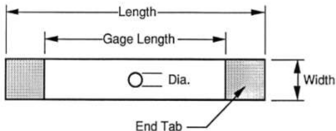
Figure 5. WVU Open Hole Tension Coupon.
