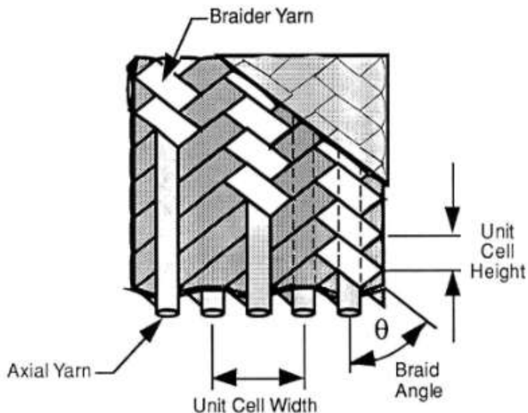
Figure 1. Illustration of a typical 2-D Triaxial Braid Configuration.
