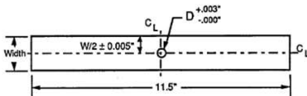
Figure 4. Boeing Straight Sided Tension Coupon.
