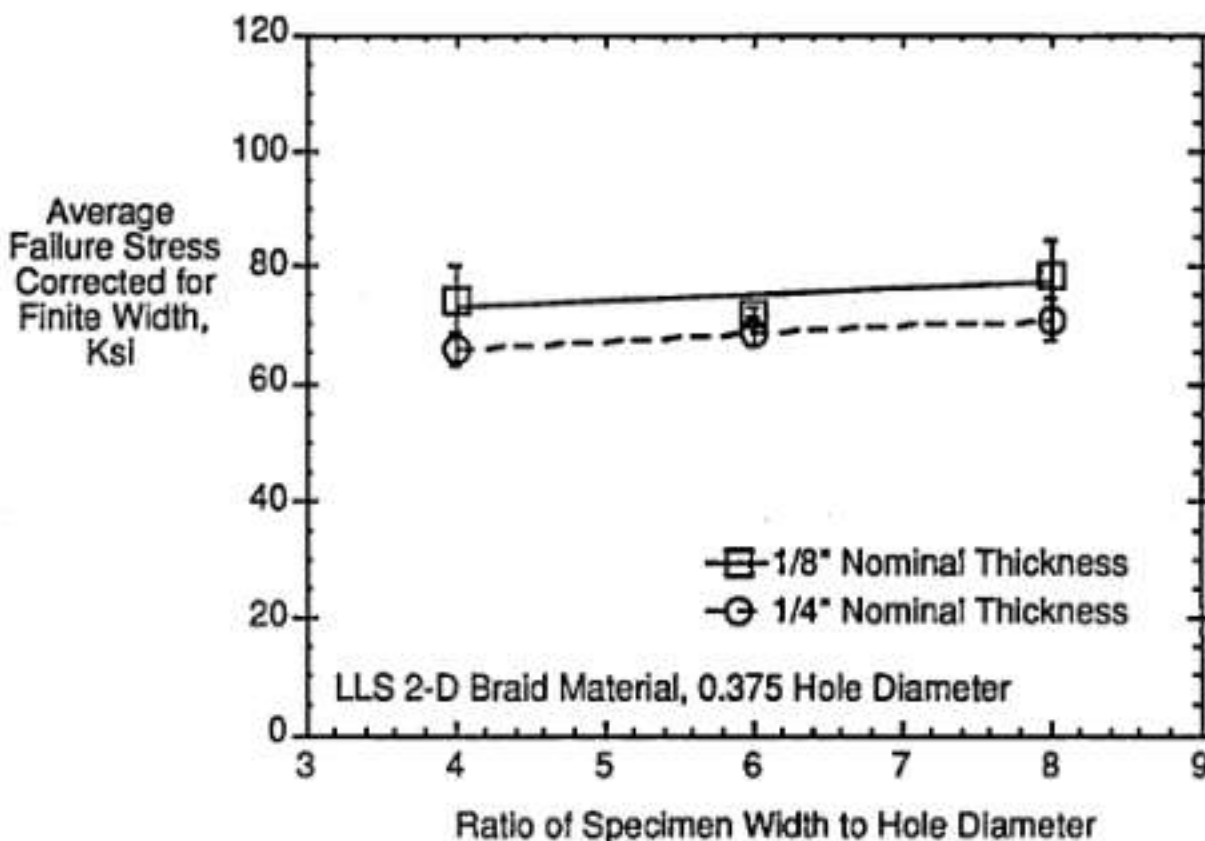
Figure 9. Effect of Specimen Thickness on Open Hole Tension Strength. LLS 2-D Braid with a 0.375 Diameter Hole.
