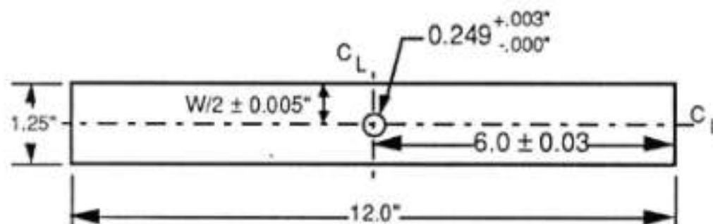
Figure 6. Lockheed Open Hole Tension Coupon.
