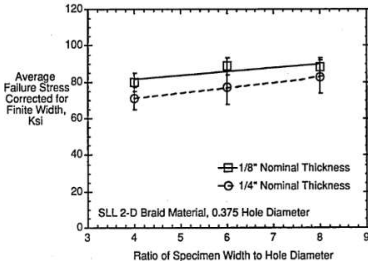
Figure 8. Effect of Specimen Thickness on Open Hole Tension Strength. SLL 2-D Braid with a 0.375 Diameter Hole.
