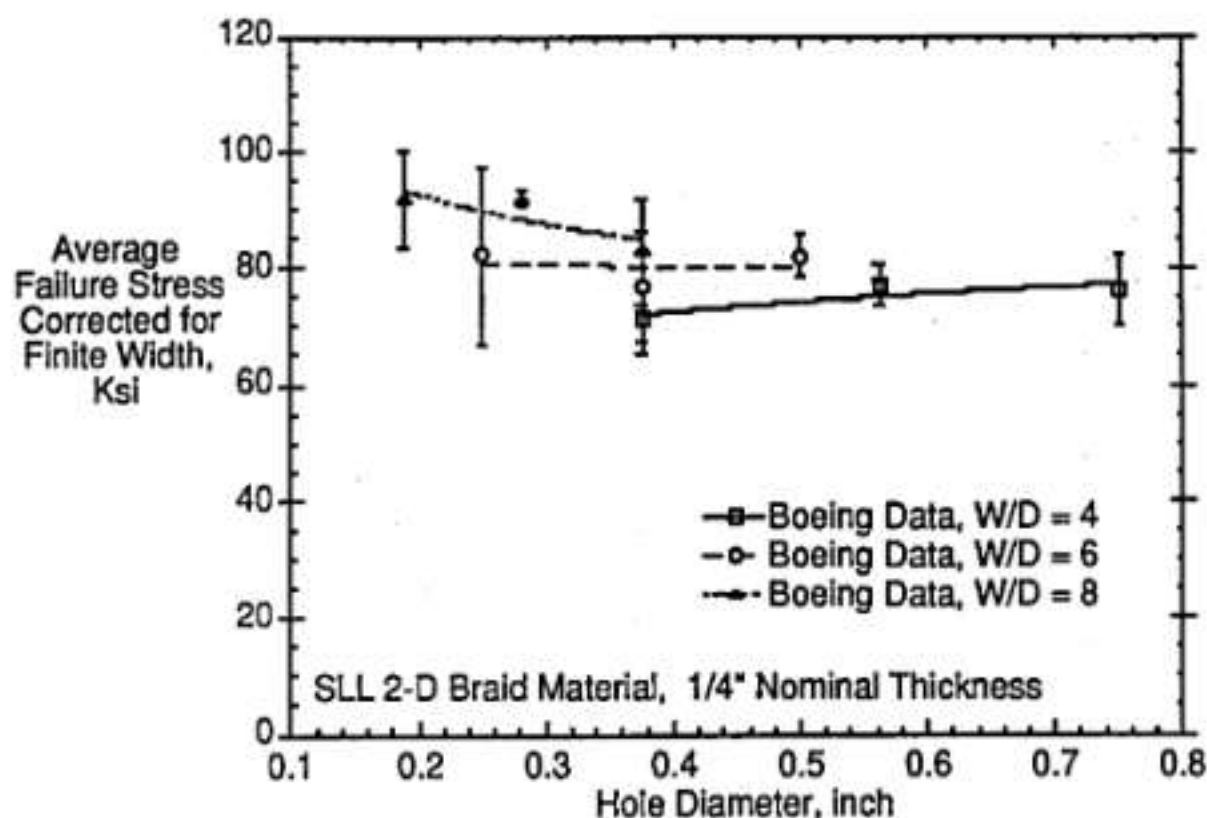
Figure 11. Effect of Hole Diameter on Open Hole Tension Strength. SLL 2-D Braid at 1/4" Nominal Thickness.
